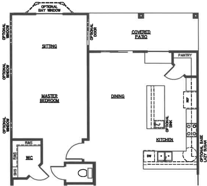
OPTIONAL KITCHEN & SITTING ROOM
